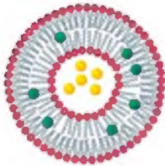
drug-loaded liposome
